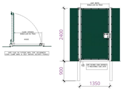
Proposed pedestrian gate
