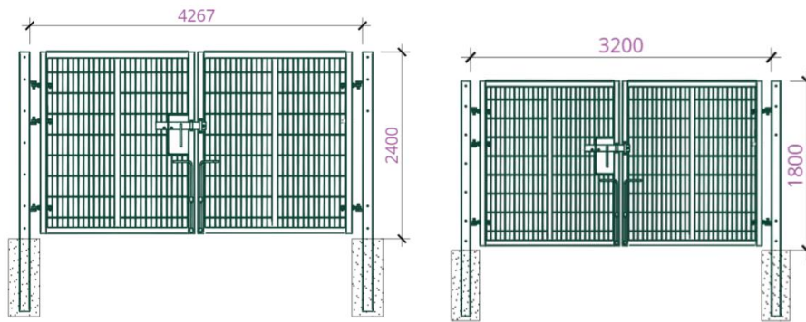
Proposed and existing vehicle gate
